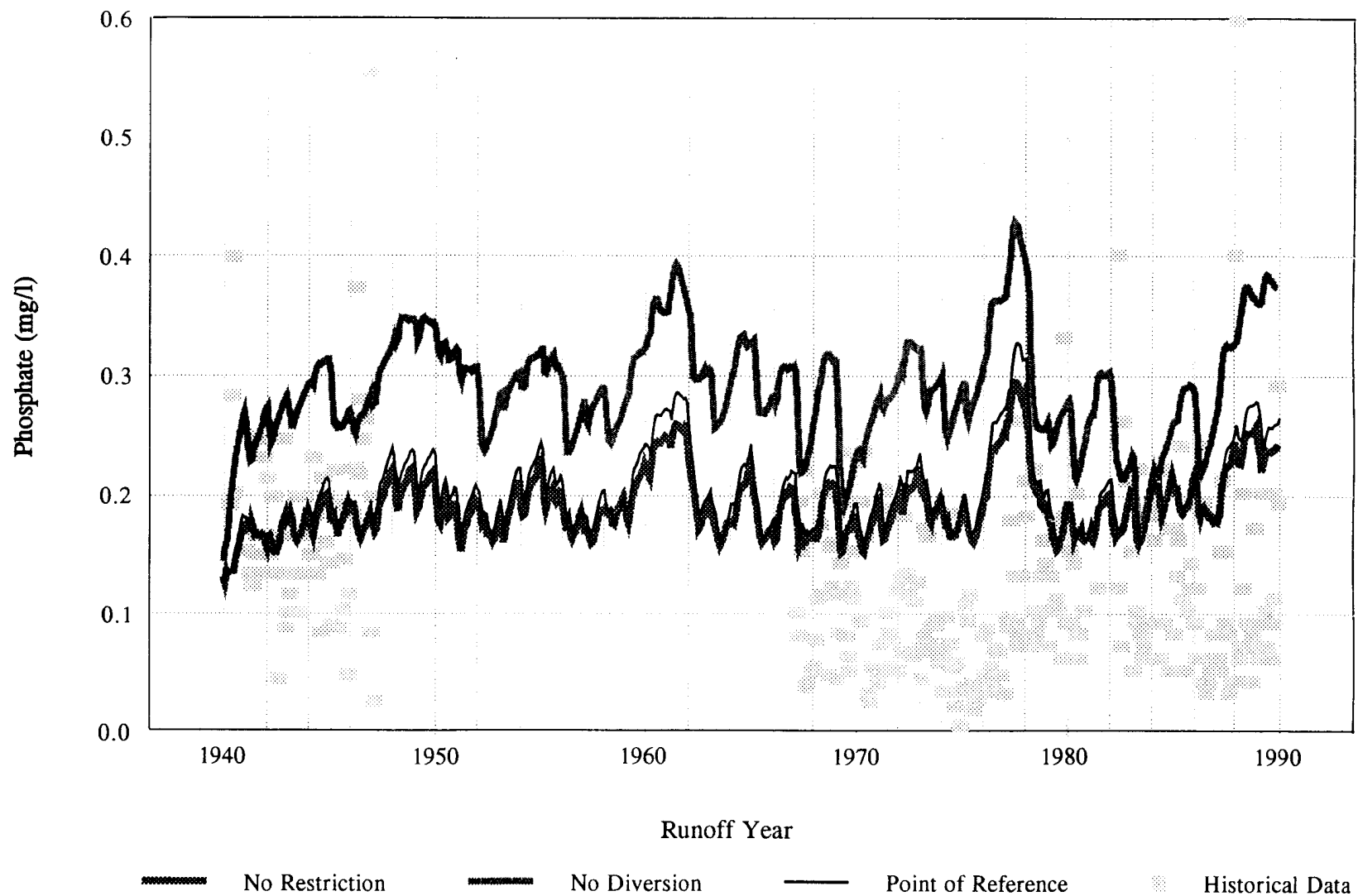
Figure 3B-15. Predicted and Historical Phosphate Concentrations for Lake Crowley Reservoir Outflow from 1940 to 1990
