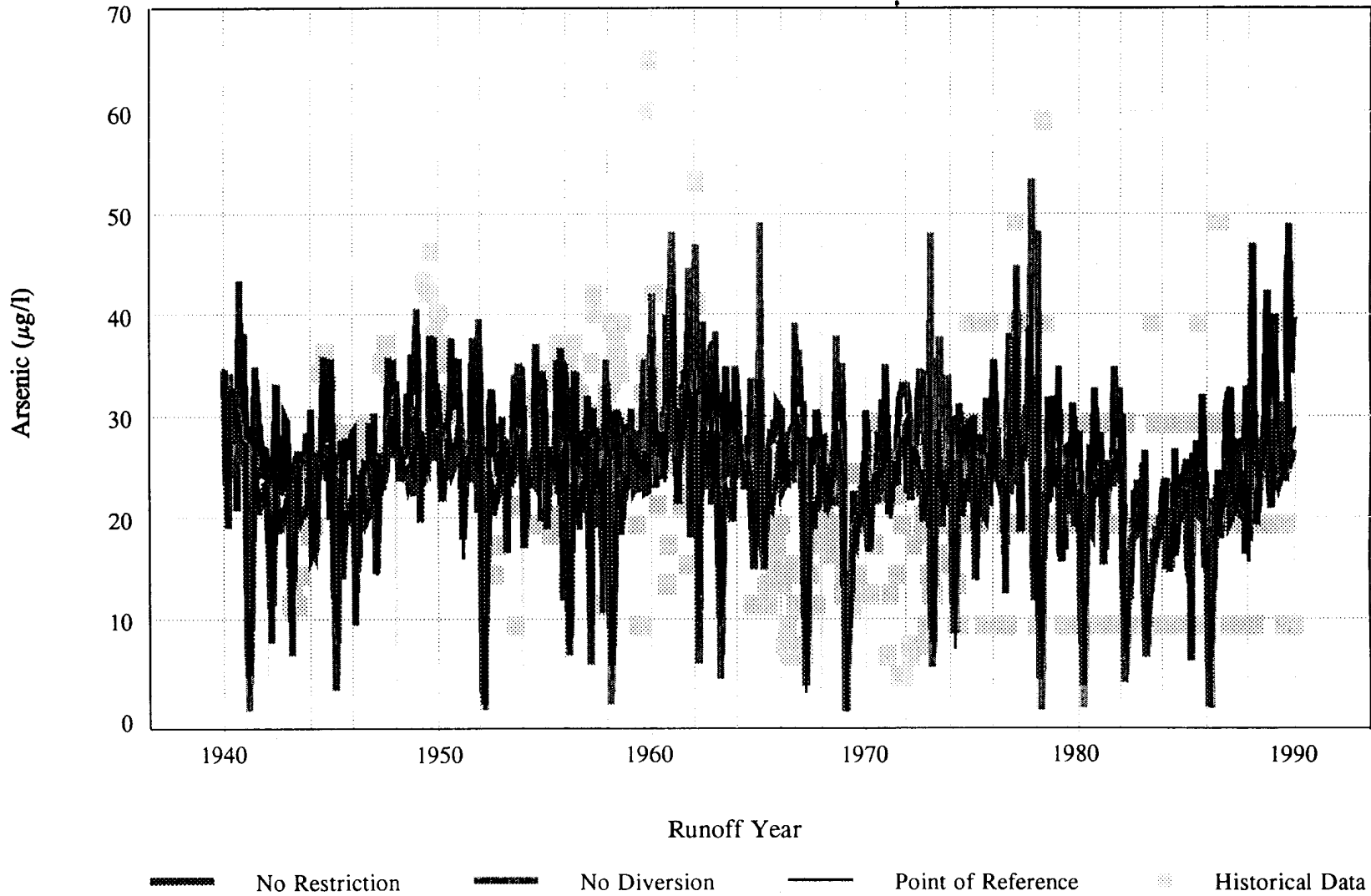
Figure 3B-10. Predicted and Historical Arsenic Concentrations for LA Aqueduct Filtration Plant Inflow from 1940 to 1990
