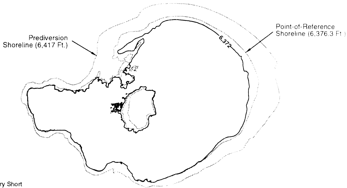
Figure 2-6. Lake Configuration at the Protected Lake Level - 6,372-Ft Alternative
