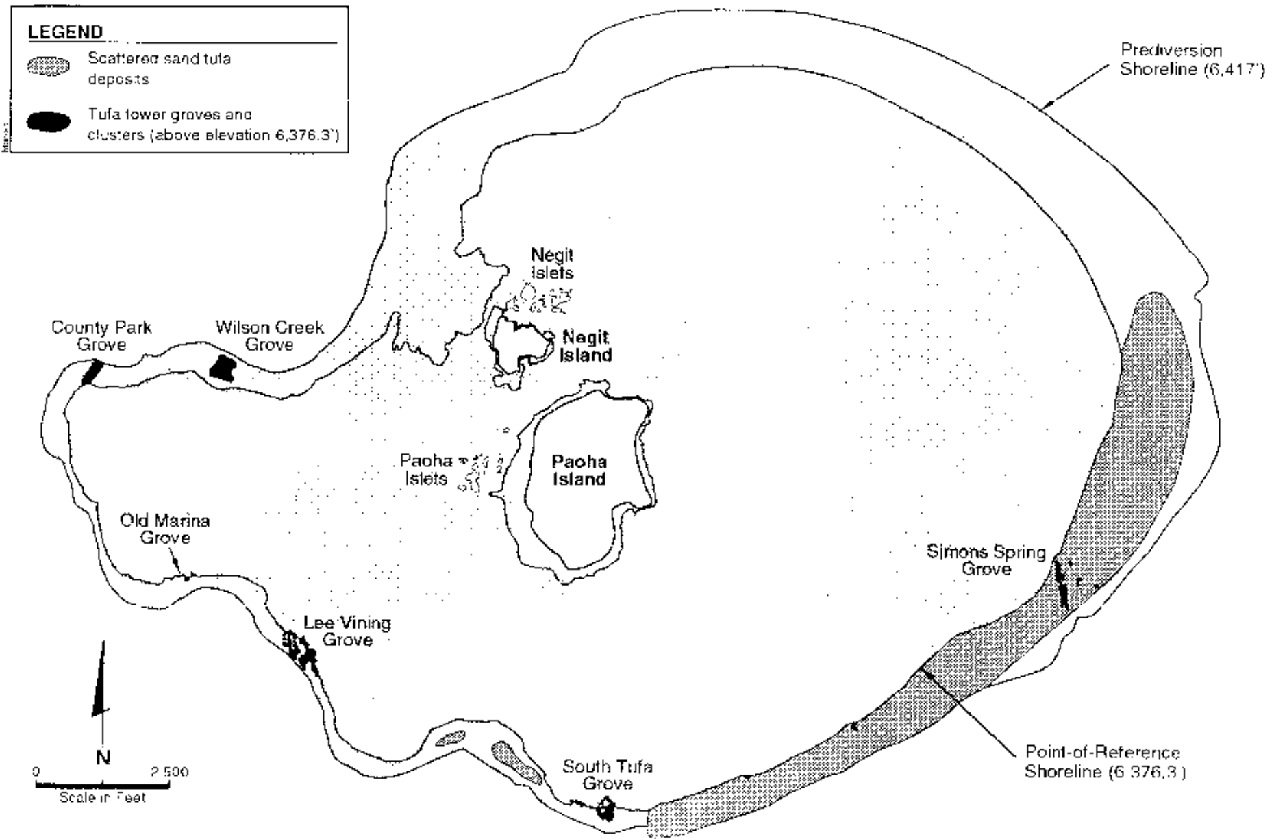
Figure 3I-9. Distribution of Tufa Deposits at Mono Lake
