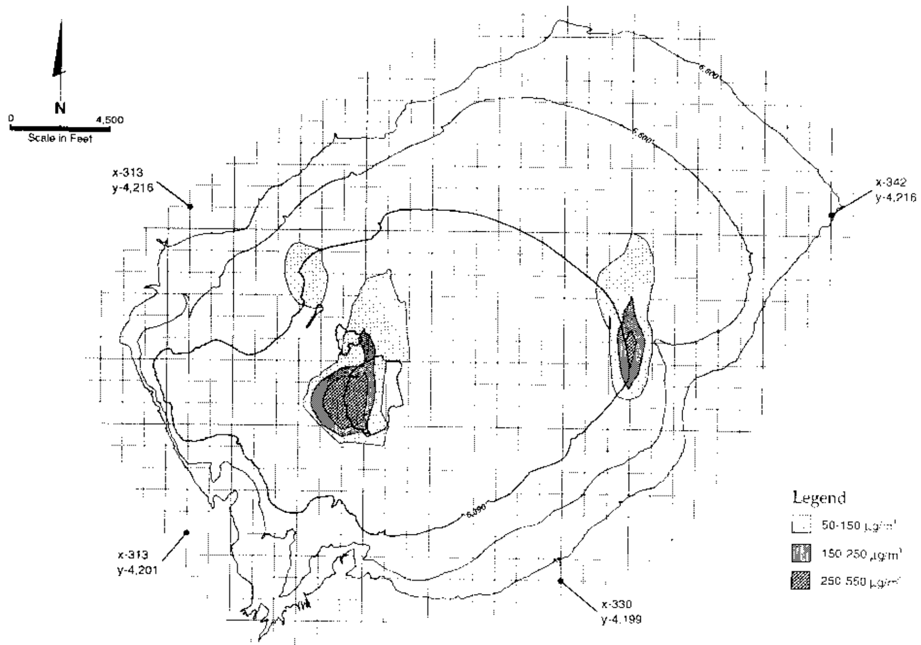
Figure 3H-31. FDM Modeling Results for a Lake Elevation of 6,390 Feet on the Maximum Episode Day
