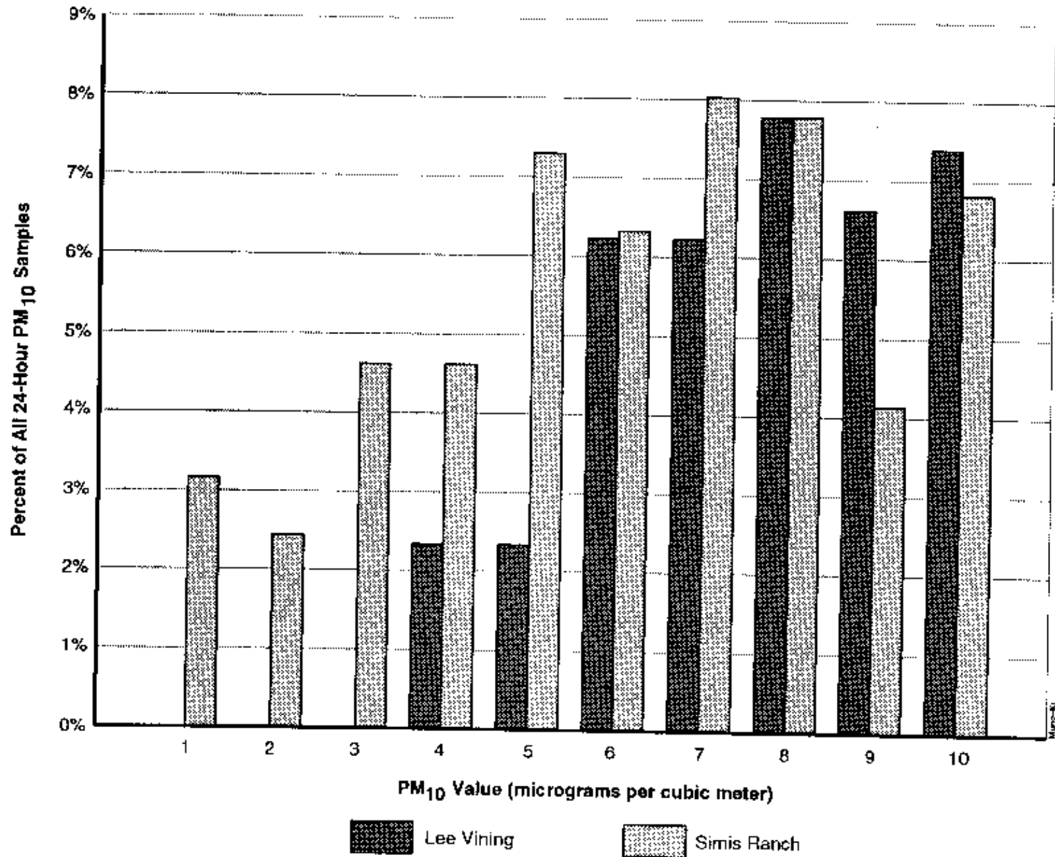
Figure 3H-13. Frequency of Low PM 10 Values at Lee Vining and Simis Ranch
