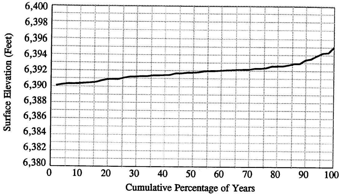
Figure 3A-20. Simulated Mono Lake Surface Elevation 6,390-Ft Alternative
